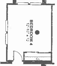
OPTIONAL BEDROOM 4 AT LOFT (WITH OPTIONAL DOOR AT BATHROOM 2)
